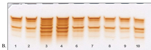
Figure 3 Changes in the activity (A) and isozymic patterns (B) of extracellular laccase in media of Cerrena unicolor cultivated 14 days with 10 dilutions of ABTS. On PAGE slab (B) the dilutions No 5 was omitted; ctrl - control. PAGE slab stained with guaiacol.
